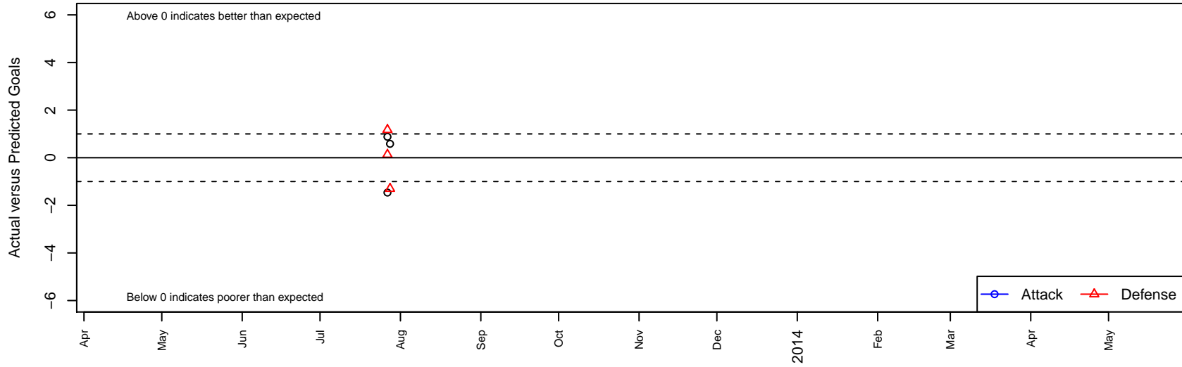
Albertson 98 B97 Dots are actual minus expected GF (blue circles) and GA (red triangles). Blue line is smoothed change in attack strength. Red is smoothed change in defense strength.
